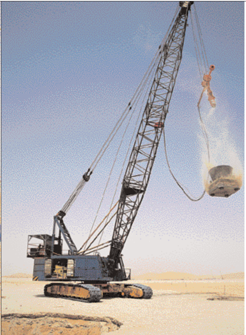
THE MARS PROCESS (MENARD AUTOMATIC RELEASE SYSTEM) optimizes the energy from ground compaction by eliminating energy loss from braking or friction.
